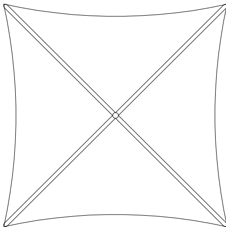
267726 SKYWAYS SINGLE POST HYPAR 16' X 16' W/10' ENTRANCE
