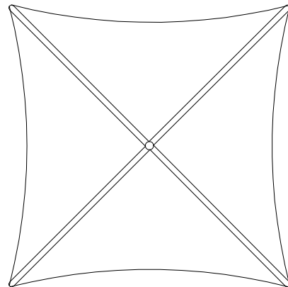
267725 SKYWAYS SINGLE POST HYPAR 14' X 14' W/10' ENTRANCE
