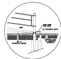
SUGGESTED RAMP BERM EXIT PLATE 8"/12" DECK TO GRADE/DB/RESILIENT SURFACING INSTALLATION REFER TO RAMP BERM EXIT PLATE INSTALLATION SHEET
